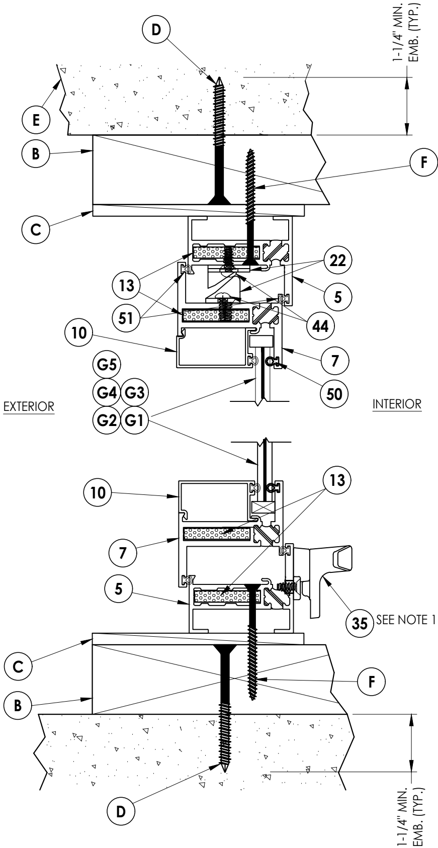
2 3 VERTICAL CROSS SECTION Shown w/ 2X Buck Construction
