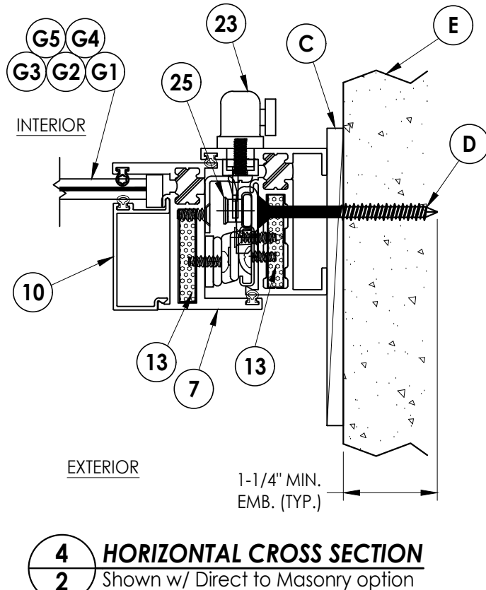
3 2 HORIZONTAL CROSS SECTION Shown w/ Steel Stud option
