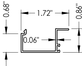
10 GLASS STOP 5/16", 7/16"
