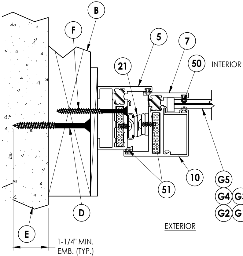
1 3 HORIZONTAL CROSS SECTION Shown w/ 2X Buck Construction
