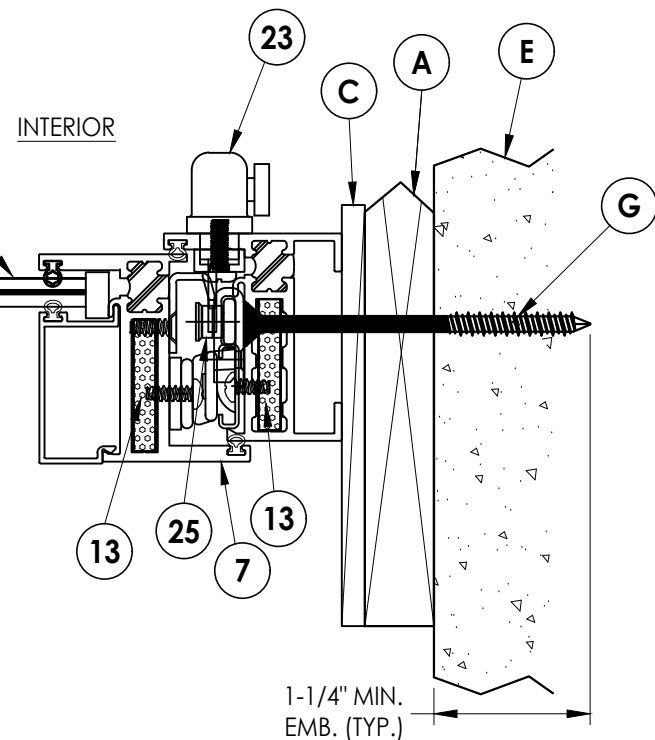
2 2 HORIZONTAL CROSS SECTION Shown w/ 1X Sub buck option
